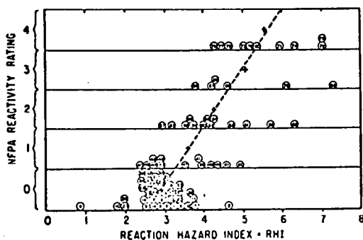
Fig 4 Correlation of the NFA Reactivity Rating with the Reaction Hazard Index (Ref 2)
